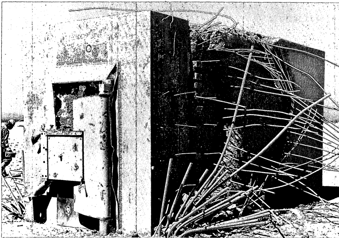
Fig. 3—Front and north faces of vault, postshot.
